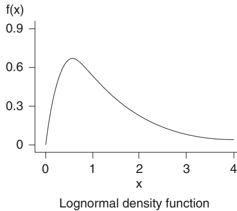
Figure 2.12.1–4 Log-normal PDF.
