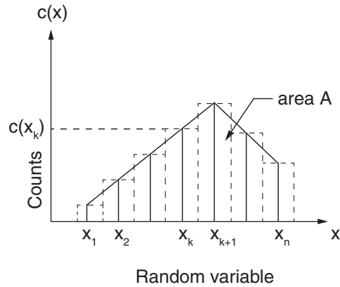
Figure 2.12.1-6 Histogram.
