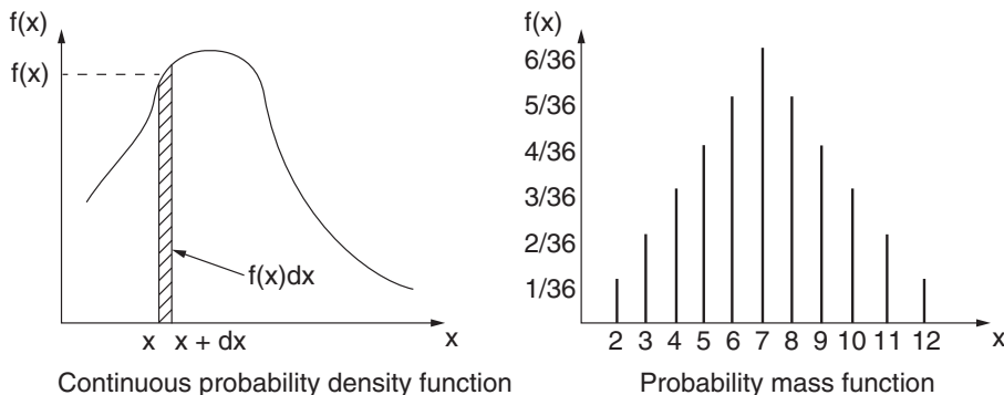
Figure 2.12.1-1 Probability distributions of continuous and discrete variables.
