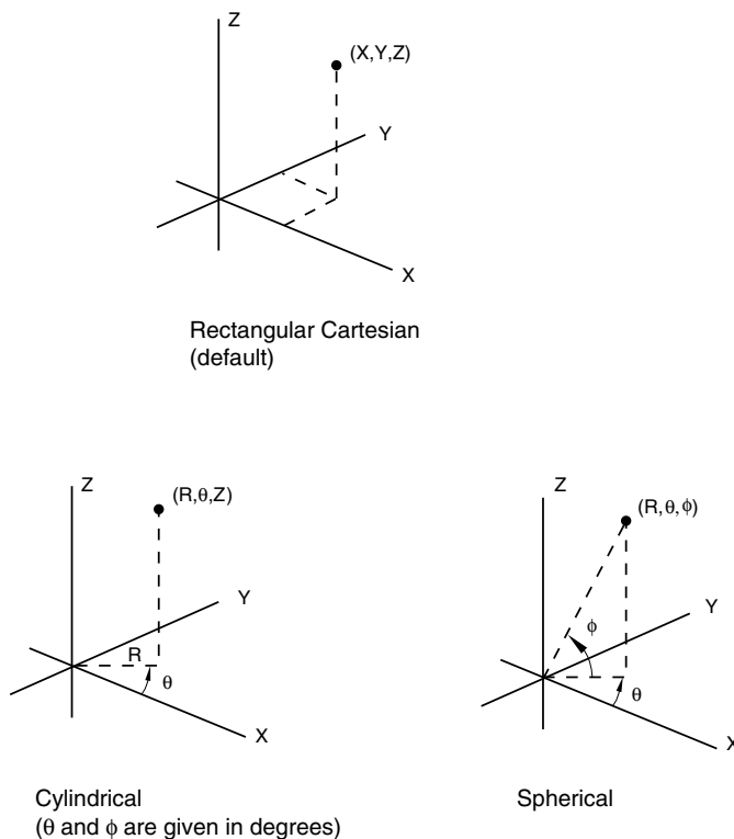
Figure 2.1.1–2 Coordinate systems.
