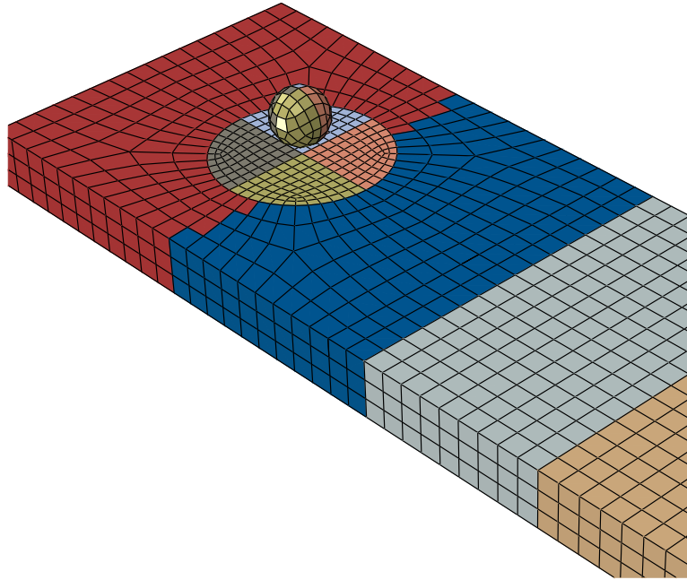
Figure 3.5.3–2 Modified domain decomposition.
