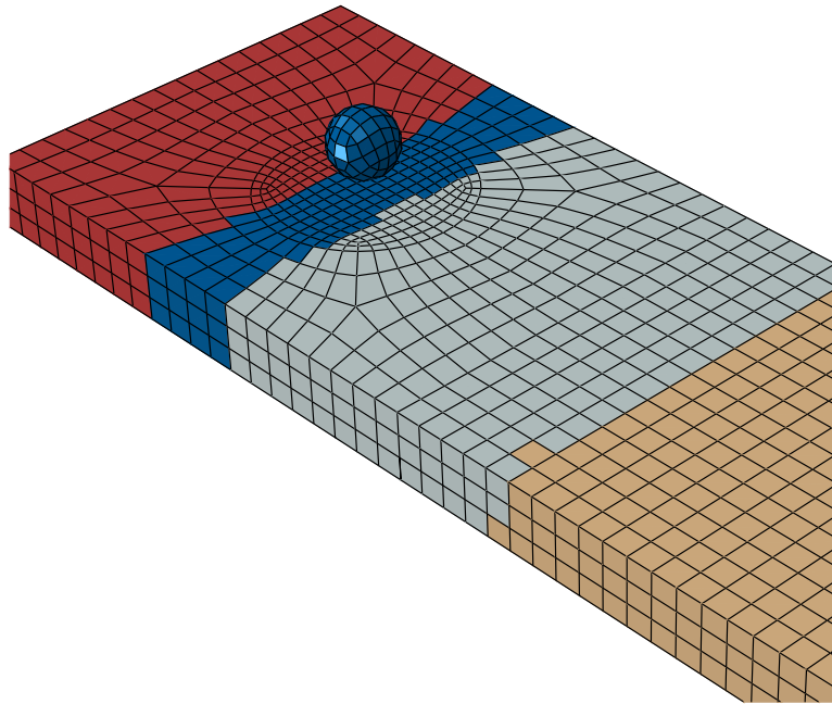
Figure 3.5.3–1 Original domain decomposition.
