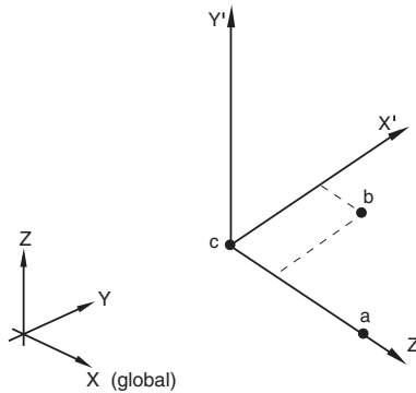
Figure 2.2.5-1 Orientation systems.
