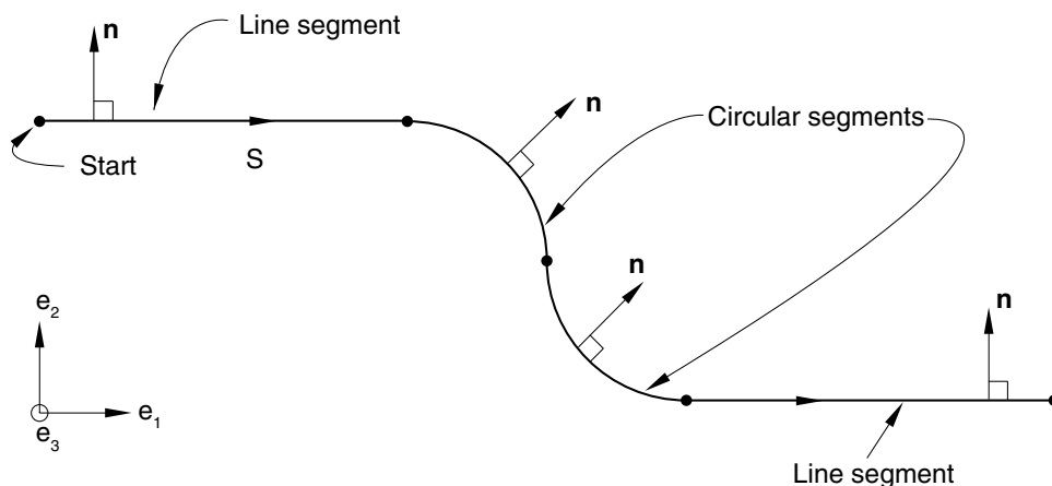
Figure 2.3.4–5 Orientation of surface normals for a rigid surface.
