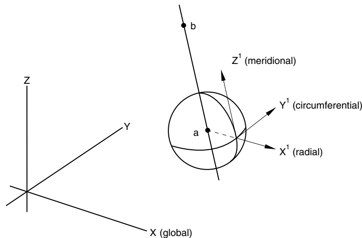
Figure 2.1.5–3 Spherical transformation.
