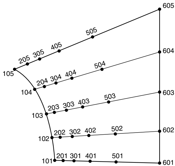
Figure 2.1.1-10 Result of bias example.
