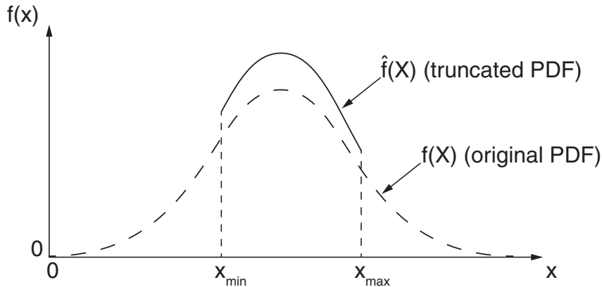
Figure 2.12.1–9 Truncated PDF.
