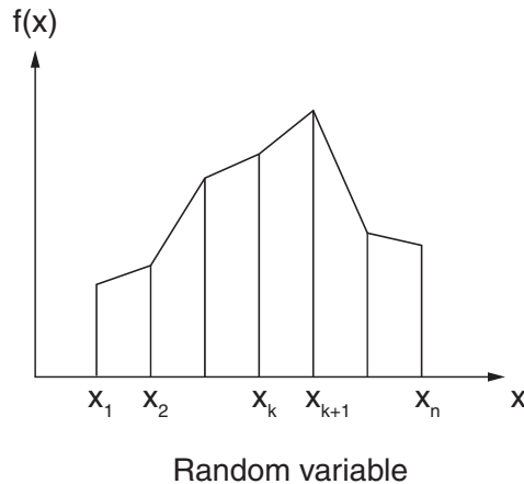
Figure 2.12.1–5 Piecewise linear PDF.
