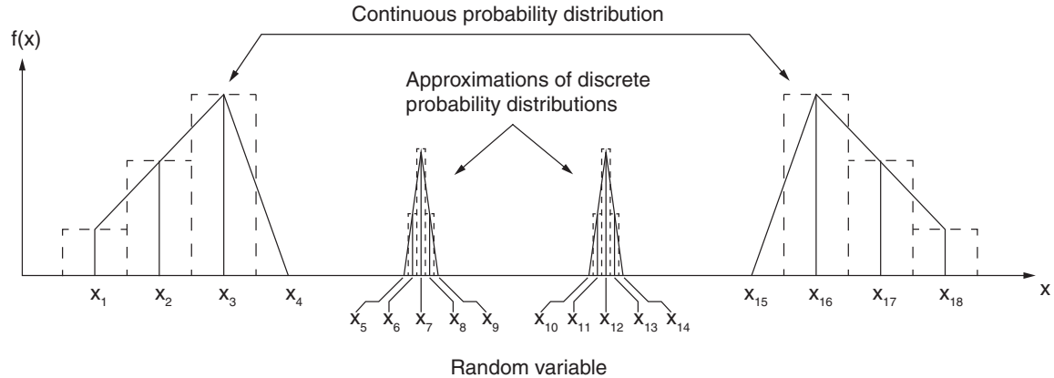
Figure 2.12.1-7 Approximating a discrete probability distribution using a piecewise linear PDF.
