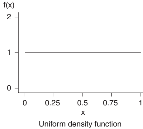
Figure 2.12.1–2 Uniform PDF.
