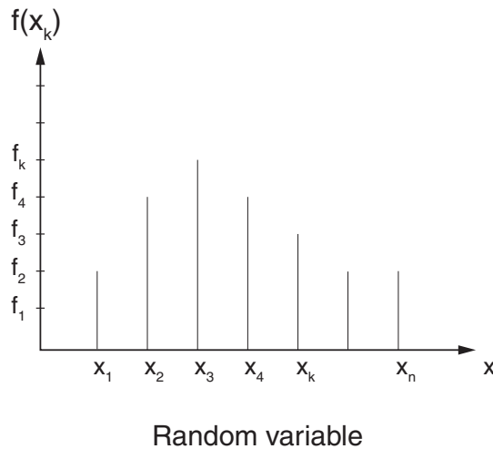
Figure 2.12.1–8 Discrete PDF.
