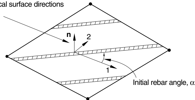
Figure 2.2.3–3 Rebar in a three-dimensional shell, membrane, or surface element.
