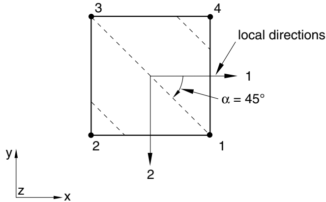
Figure 2.2.3-5 Rebar defined relative to default local coordinate directions.
