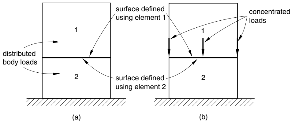
Figure 4.1.3-3 Invalid section definitions.
