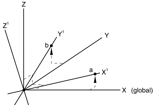
Figure 2.1.5–1 Cartesian transformation.
