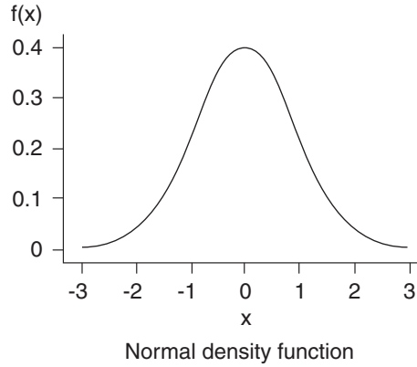
Figure 2.12.1–3 Normal PDF.
