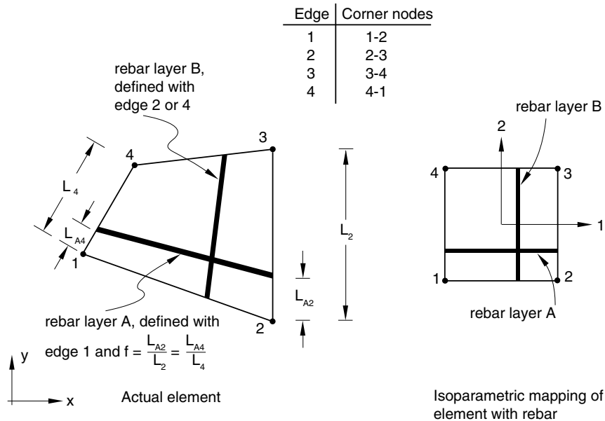
Figure 2.2.4-9 Isoparametric rebar layer definition in solid elements.
