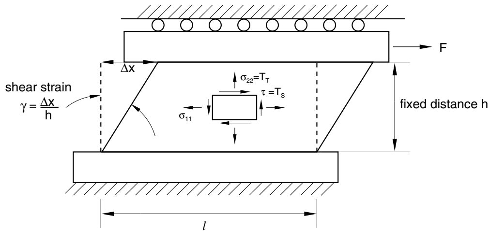
Figure 22.5.2–3 Simple shear test.
