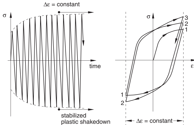
Figure 23.2.2–4 Plastic shakedown.
