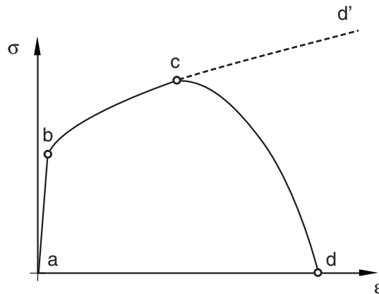
Figure 24.1.1–1 Typical uniaxial stress-strain response of a metal specimen.
