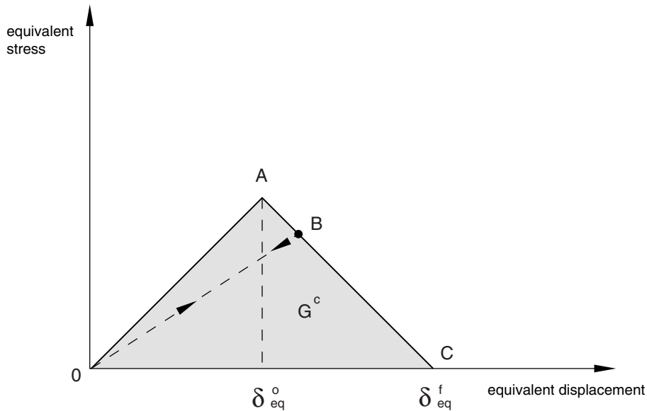
Figure 24.3.3–3 Linear damage evolution.
