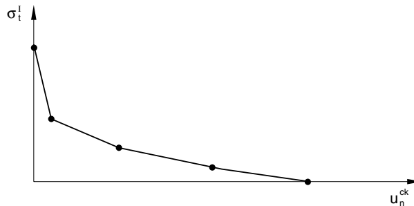
Figure 23.6.2–2 Postfailure stress-displacement curve.
