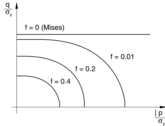
Figure 23.2.9–1 Schematic of the yield surface in the p – q plane.
