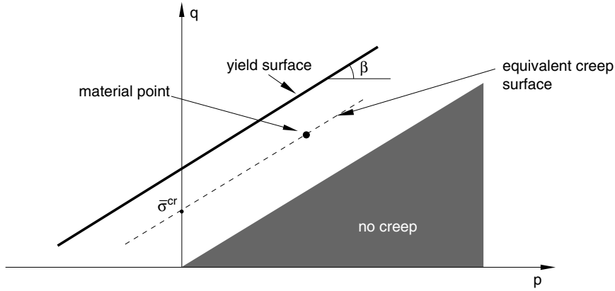
Figure 23.3.1–13 Equivalent creep stress defined as the shear stress.
