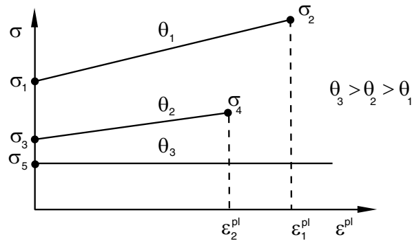
Figure 23.2.5-1 Stress versus plastic strain behavior.
