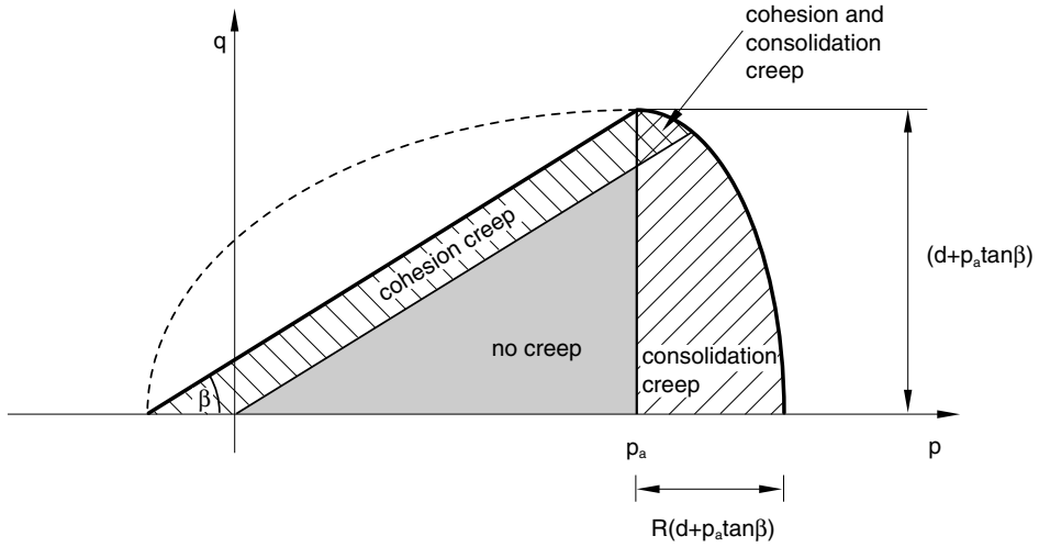
Figure 23.3.2-5 Regions of activity of creep mechanisms.
