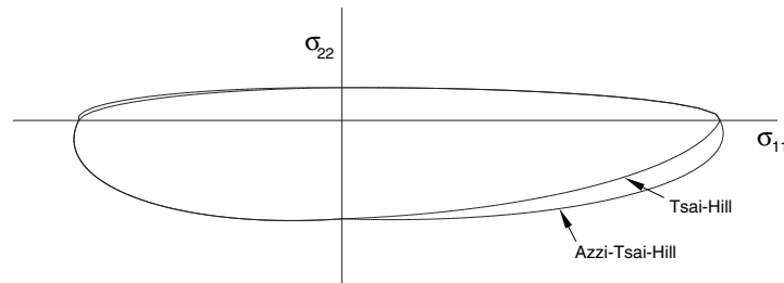
Figure 22.2.3-3 Tsai-Hill versus Azzi-Tsai-Hill failure envelope ( I_F = 1.0 ).
