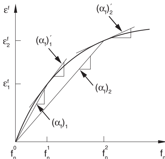
Figure 26.1.3–1 Definition of the field expansion coefficient.
