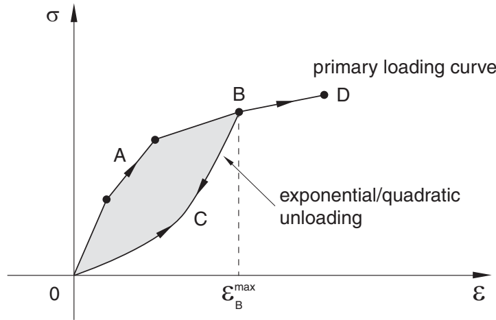
Figure 23.4.1-4 Exponential/quadratic unloading.
