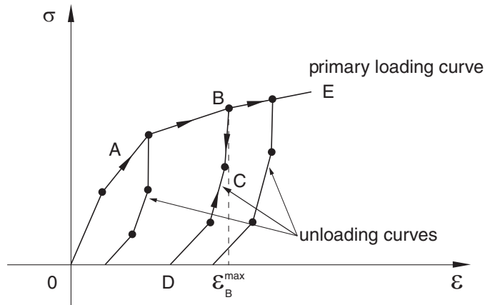
Figure 23.4.1–8 Interpolated curve unloading.
