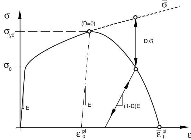
Figure 24.2.3-1 Stress-strain curve with progressive damage degradation.
