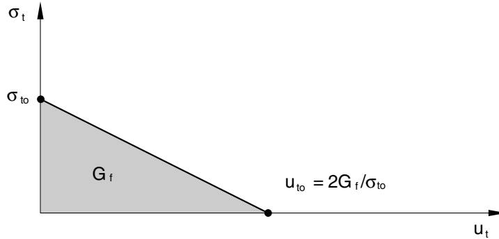
Figure 23.6.3–5 Postfailure stress-fracture energy curve.
