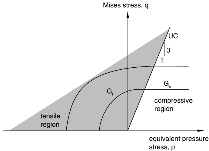
Figure 23.2.10-2 Schematic of the flow potentials in the p - q plane.
