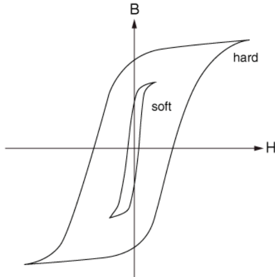
Figure 26.5.3–1 Response of hard and soft magnetic materials.
