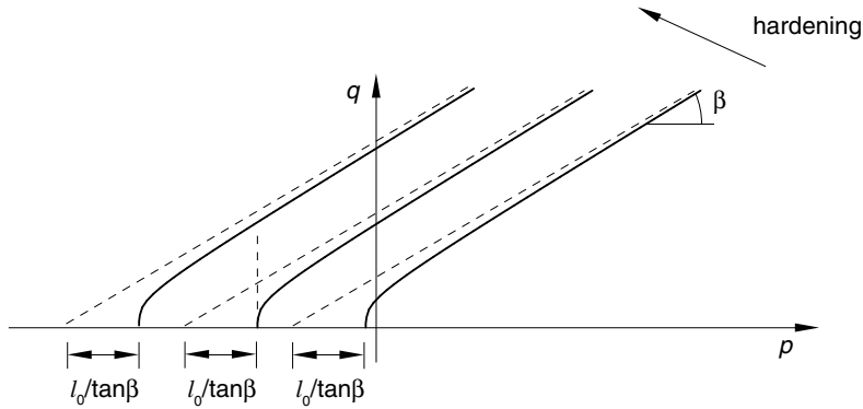
Figure 23.3.1–4 Hyperbolic model: yield surface and hardening in the p - q plane.
