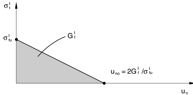
Figure 23.6.2-3 Postfailure stress-fracture energy curve.
