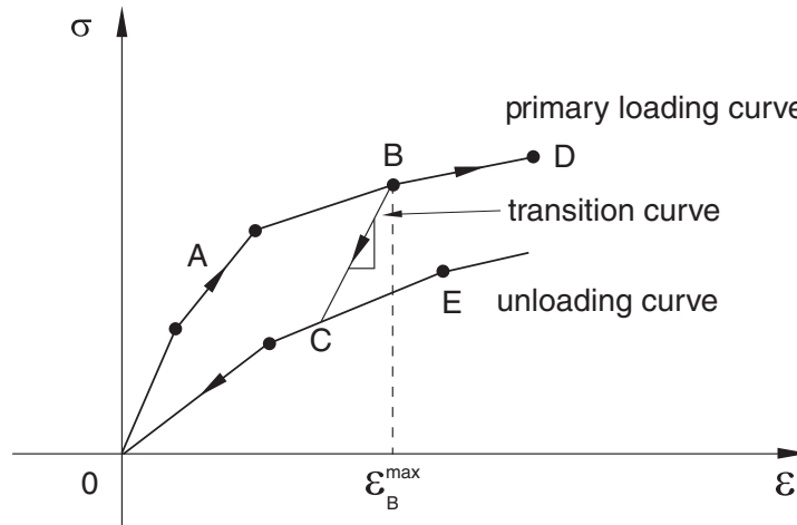
Figure 23.4.1-6 Combined unloading.
