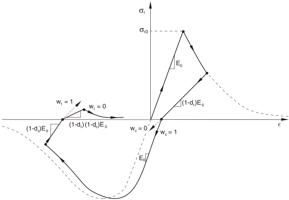
Figure 23.6.3-7 Uniaxial load cycle (tension-compression-tension) assuming default values for the stiffness recovery factors: w_t = 0 and w_c = 1 .
