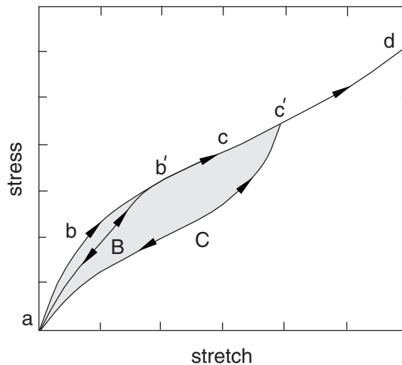
Figure 22.6.1–1 Idealized response of the Mullins effect model.
