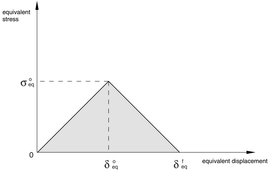
Figure 24.3.3-1 Equivalent stress versus equivalent displacement.
