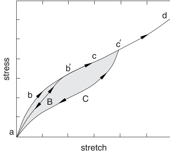
Figure 22.6.2-1 Typical stress-stretch response of an elastomeric foam material with energy dissipation.
