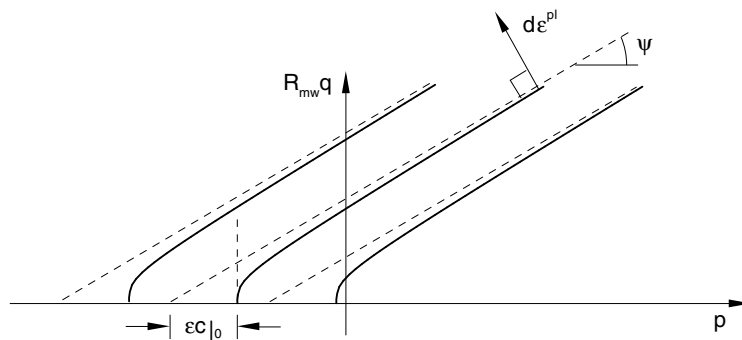
Figure 23.3.3–3 Family of hyperbolic flow potentials in the meridional stress plane.
