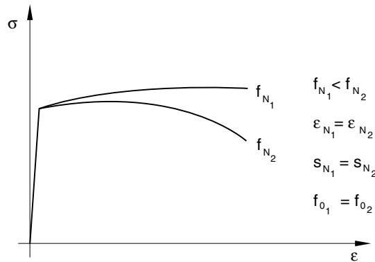
Figure 23.2.9–4 Softening (in uniaxial tension) as a function of f_N .
