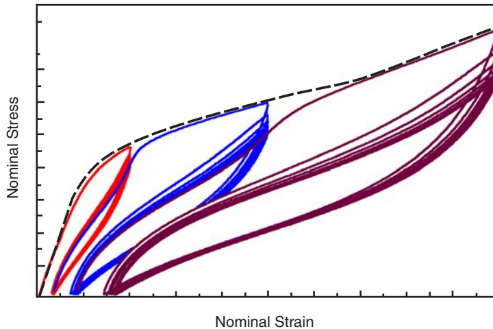
Figure 22.6.1–4 Typical available test data for Mullins effect.
