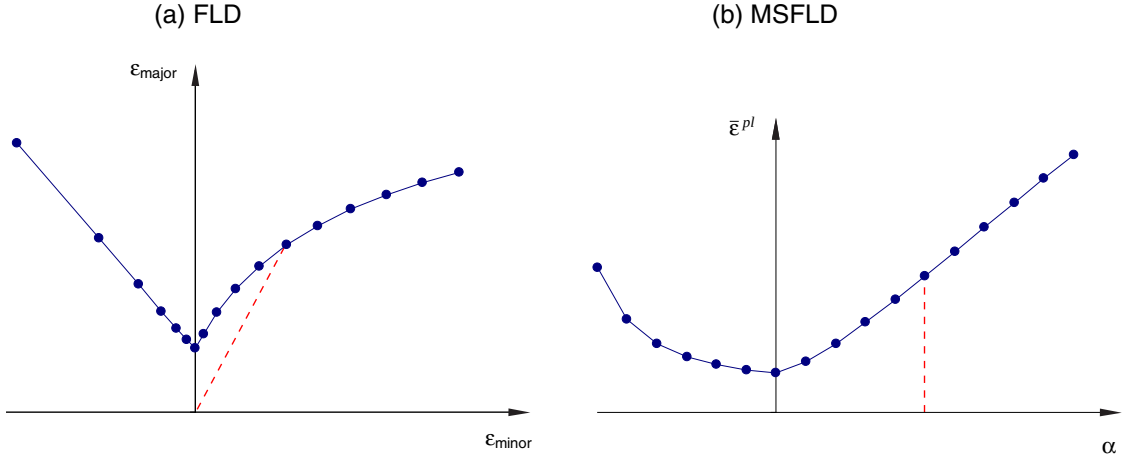
Figure 24.2.2-3 Transformation of the forming limit curve from traditional FLD representation (a) to MSFLD representation (b). Linear deformation paths transform onto vertical paths.
