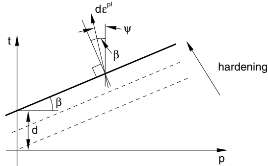
Figure 23.3.1-3 Linear Drucker-Prager model: yield surface and flow direction in the p - t plane.
