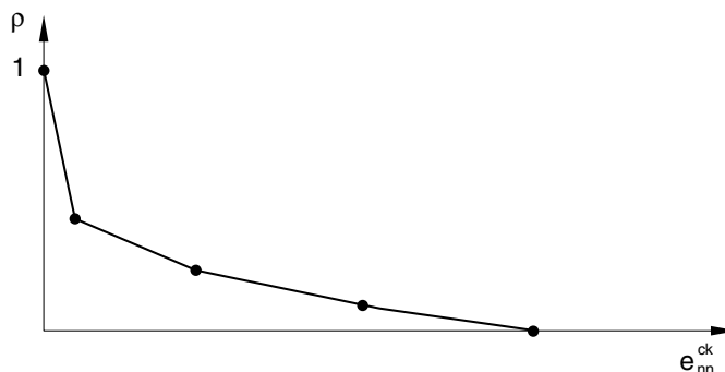
Figure 23.6.2–4 Piecewise linear form of the shear retention model.
