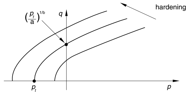
Figure 23.3.1–5 General exponent model: yield surface and hardening in the p - q plane.
