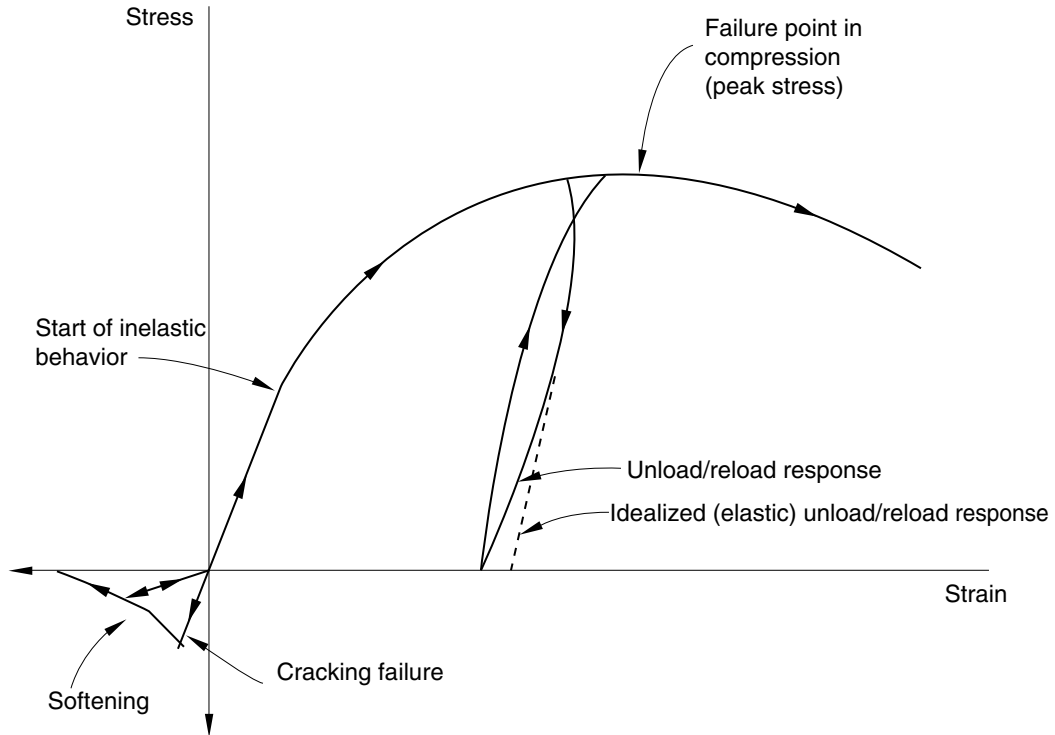
Figure 23.6.1-3 Uniaxial behavior of plain concrete.
