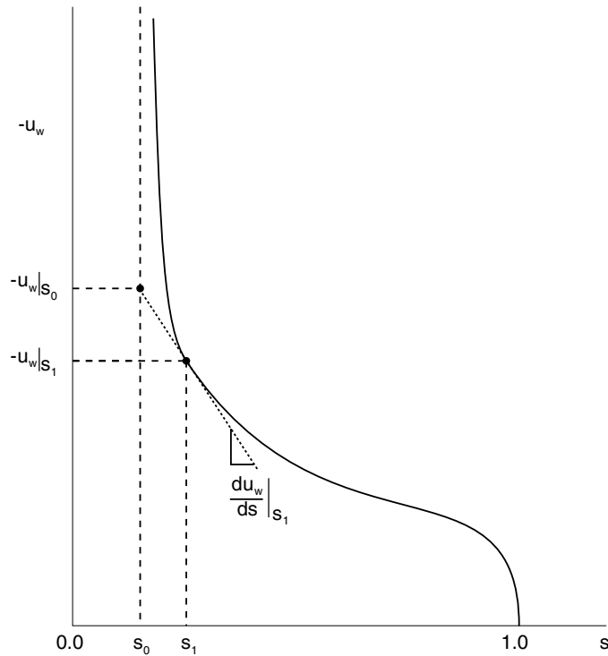
Figure 26.6.4–2 Logarithmic form of absorption and exsorption behaviors.
