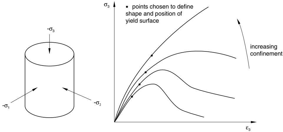
Figure 23.3.1-7 Triaxial tests with stress-strain curves for typical geological materials at different levels of confinement.
