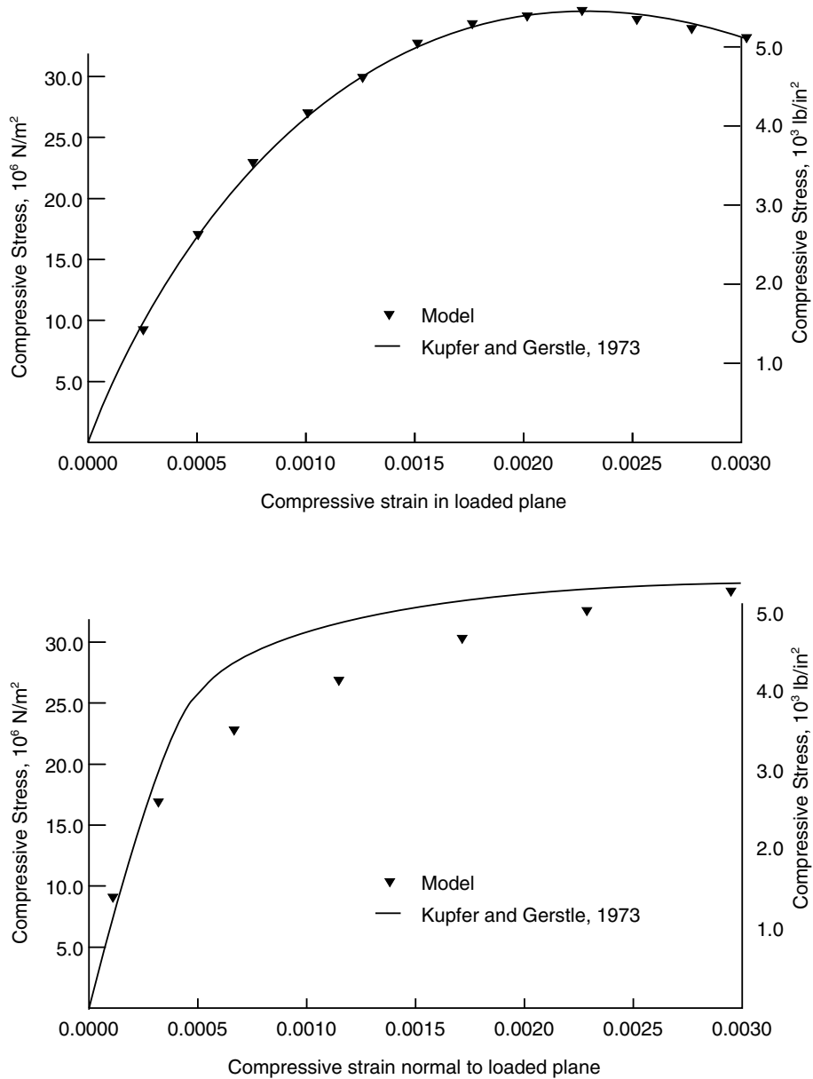
Figure 23.6.1–7 Comparison of model prediction and Kupfer and Gerstle's data for a biaxial compression test.
