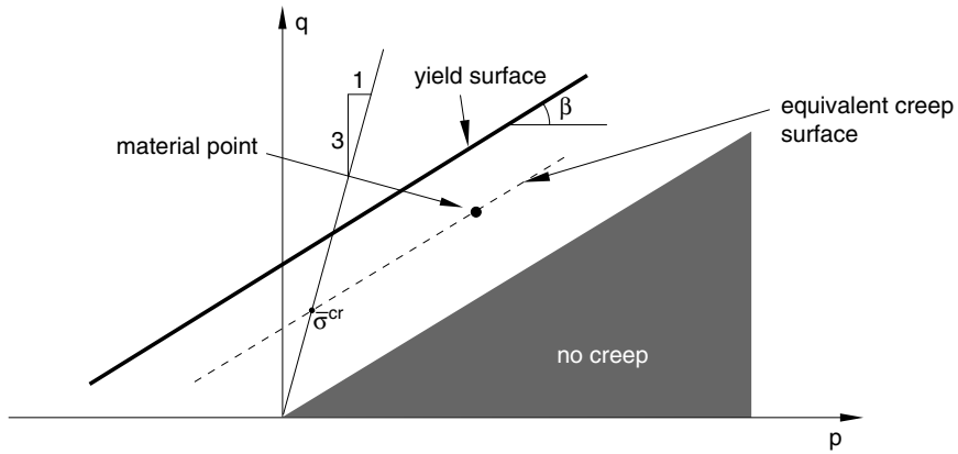
Figure 23.3.2-6 Equivalent creep stress for cohesion creep.
