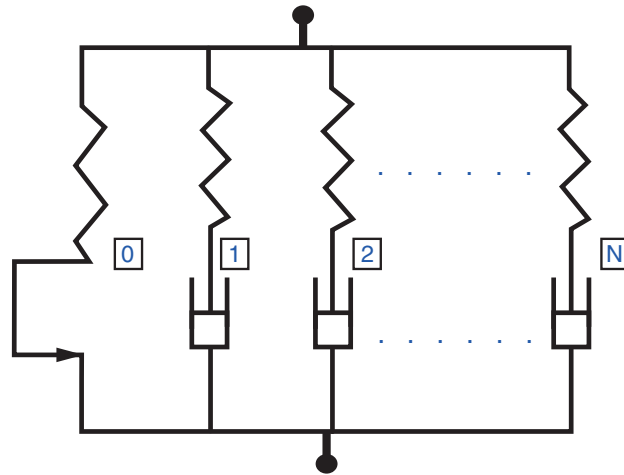
Figure 22.8.2–1 Nonlinear viscoelastic-elastoplastic model with multiple parallel networks.
