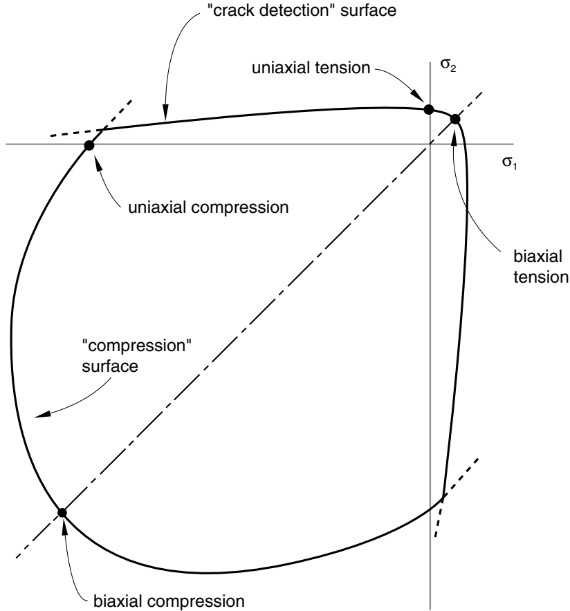
Figure 23.6.1–4 Yield and failure surfaces in plane stress.
