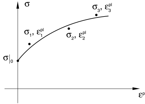
Figure 23.2.2-8 Half cycle of stress-strain data.
