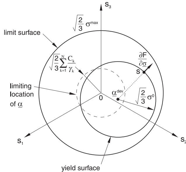
Figure 23.2.2-3 Three-dimensional representation of the hardening in the nonlinear isotropic/kinematic model.
