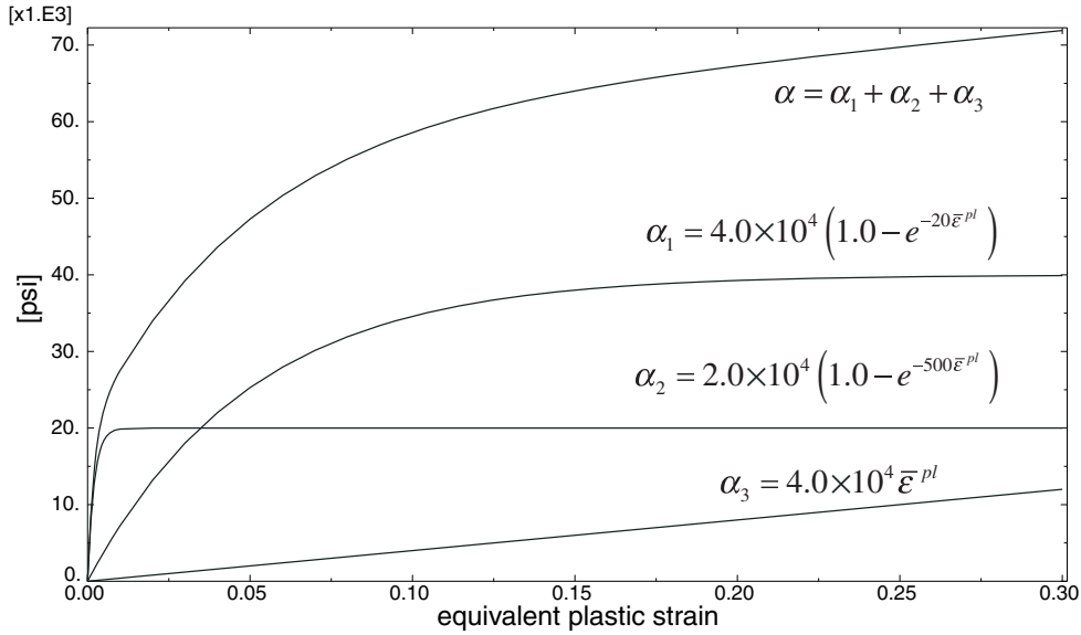
Figure 23.2.2-1 Kinematic hardening model with three backstresses.
