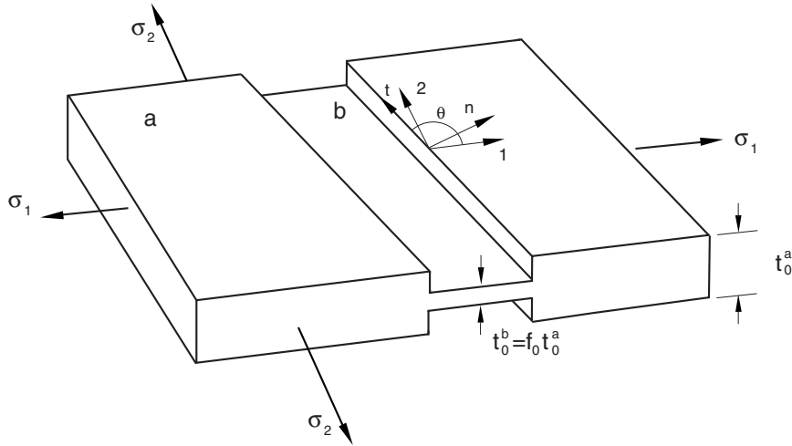
Figure 24.2.2-2 Imperfection model for the M-K analysis.
