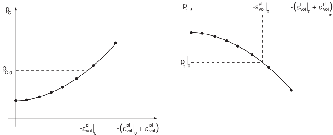
Figure 23.3.4–4 Typical piecewise linear clay hardening/softening curve.
