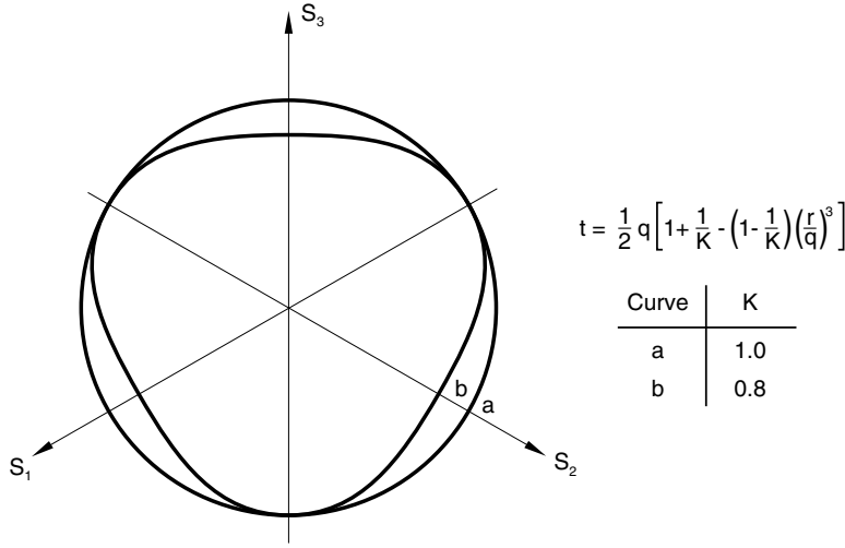
Figure 23.3.1-2 Typical yield/flow surfaces of the linear model in the deviatoric plane.
