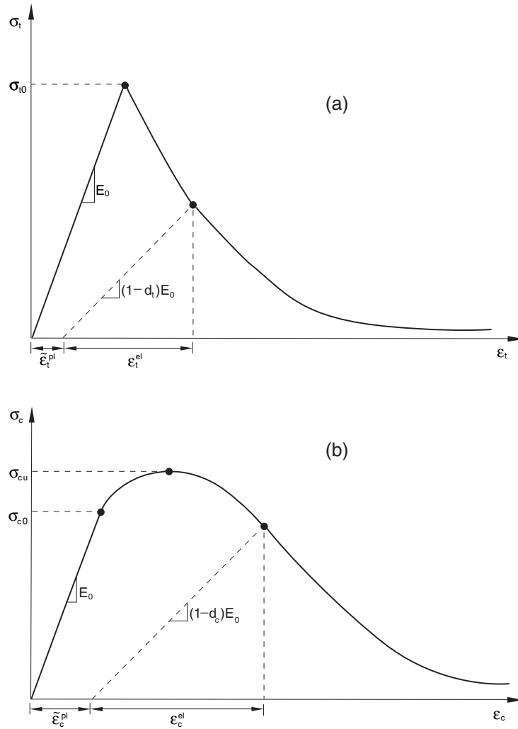
Figure 23.6.3-1 Response of concrete to uniaxial loading in tension (a) and compression (b).
