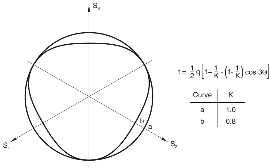
Figure 23.3.4-2 Isotropic clay yield surface sections in the \Pi -plane ( \hat{t} = t and \tilde{q} = q for the isotropic yield function).
