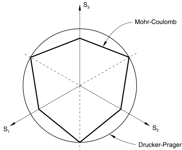
Figure 23.3.1–12 Mohr-Coulomb model in the deviatoric plane.
