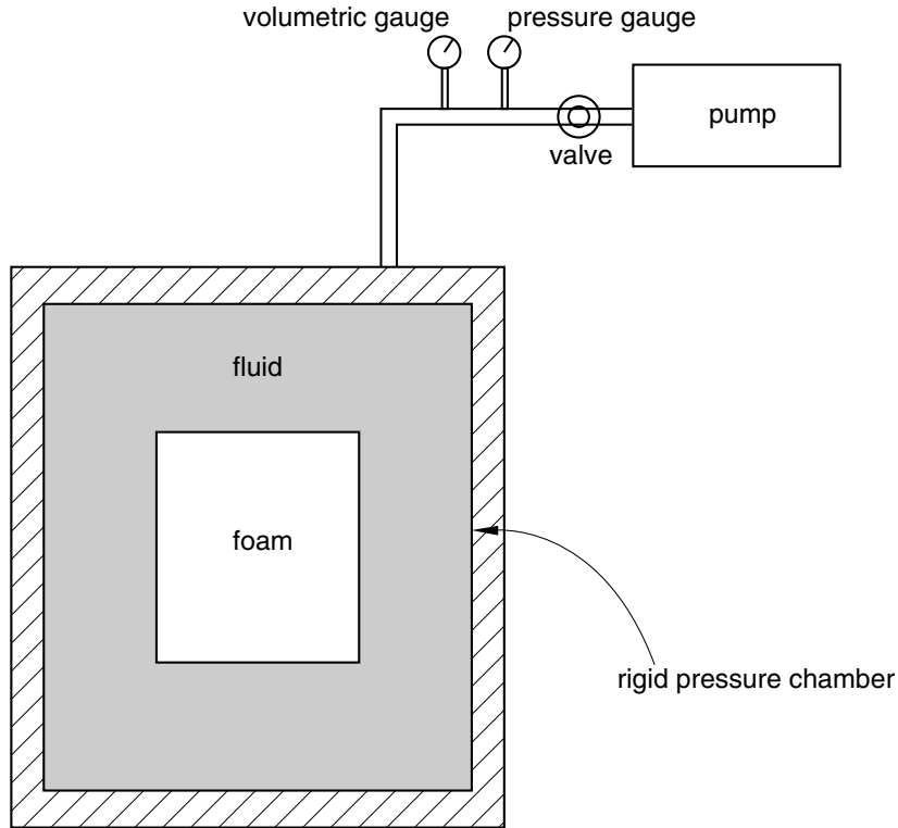
Figure 22.5.2–4 Volumetric compression test.
