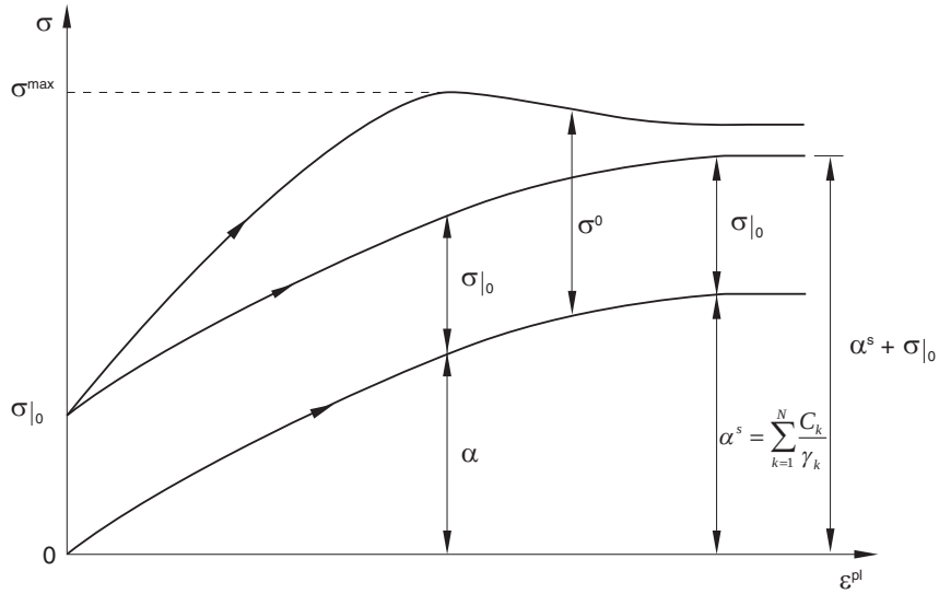
Figure 23.2.2-2 One-dimensional representation of the hardening in the nonlinear isotropic/kinematic model.
