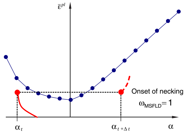
Figure 24.2.2-4 Illustration of how a sudden change in the straining direction, from \alpha_t to \alpha_{t+\Delta t} , can produce a horizontal intersection with the limit curve and lead to onset of necking.
