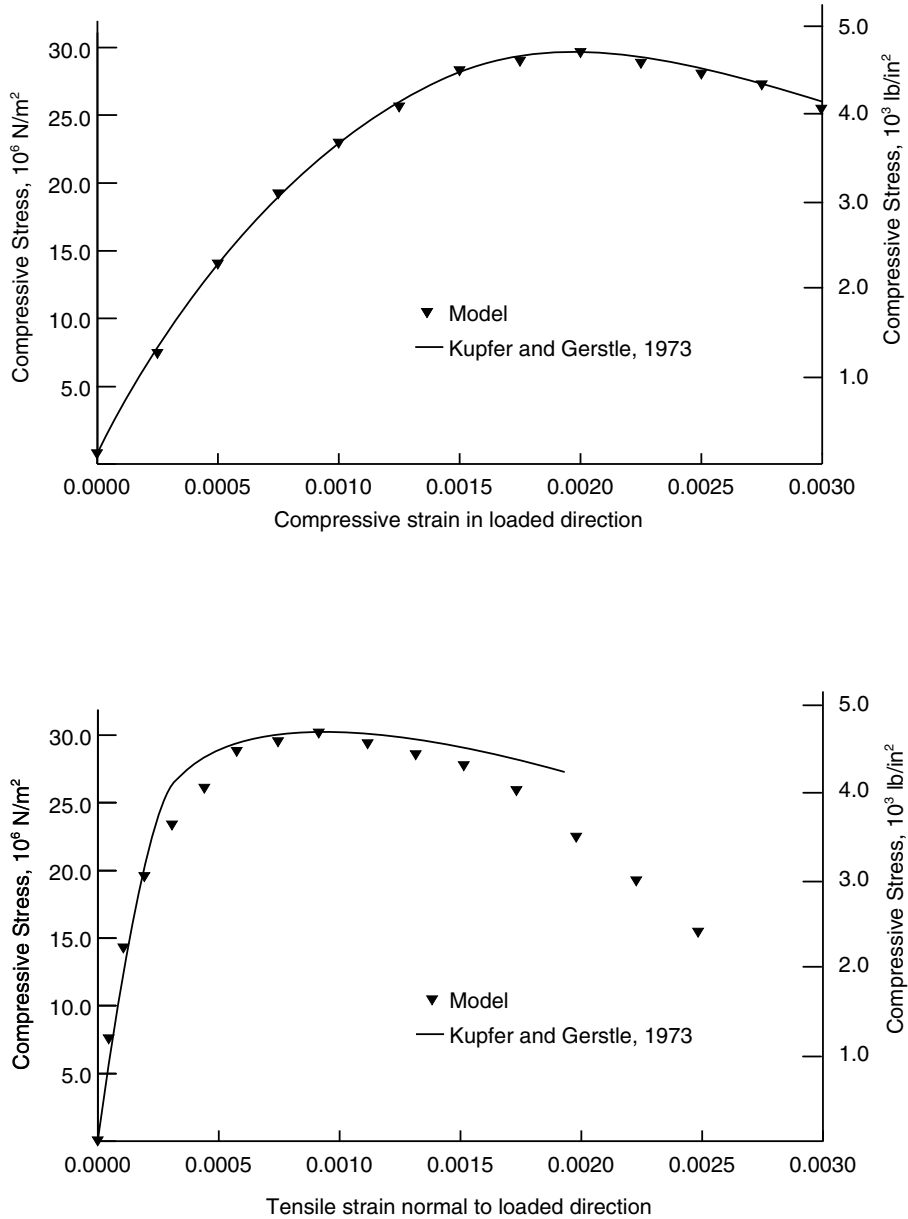
Figure 23.6.1-6 Comparison of model prediction and Kupfer and Gerstle's data for a uniaxial compression test.
