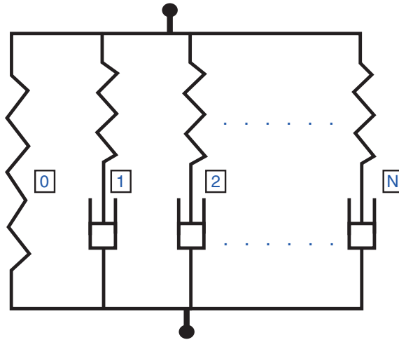
Figure 22.8.2-3 Nonlinear viscoelastic model with multiple parallel networks.
