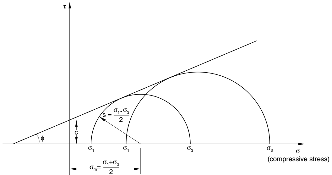
Figure 23.3.3–1 Mohr-Coulomb yield model.
