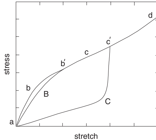
Figure 22.6.1-2 Overly stiff response at the initiation of unloading.
