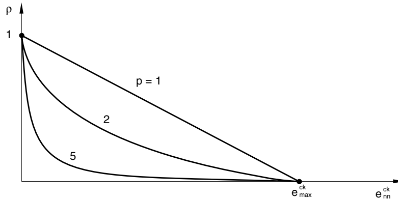
Figure 23.6.2-5 Power law form of the shear retention model.
