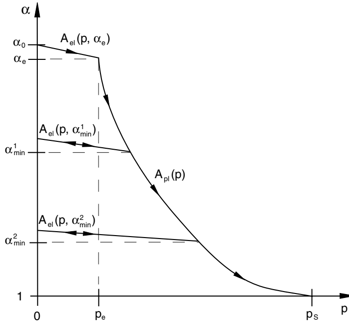
Figure 25.2.1–2 P - \alpha elastic and plastic curves for the description of compaction of ductile porous materials.
