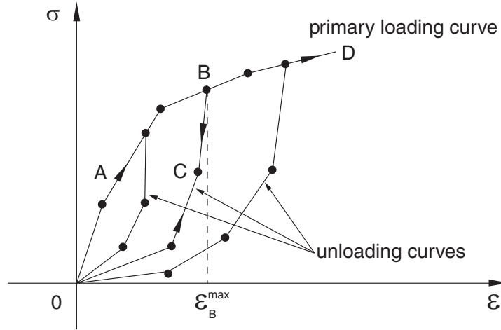
Figure 23.4.1-5 Interpolated curve unloading.
