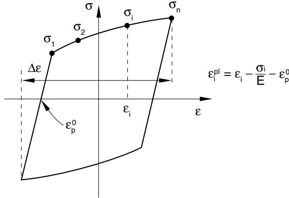
Figure 23.2.2–9 Stress-strain data for a stabilized cycle.
