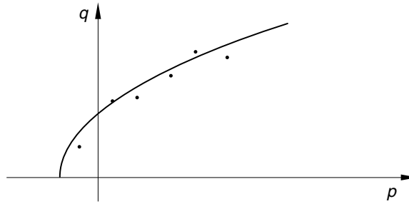
Figure 23.3.1-8 Yield surface in meridional plane.
