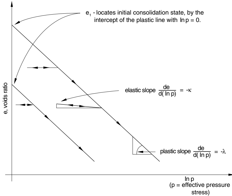
Figure 23.3.4–3 Pure compression behavior for clay model.
