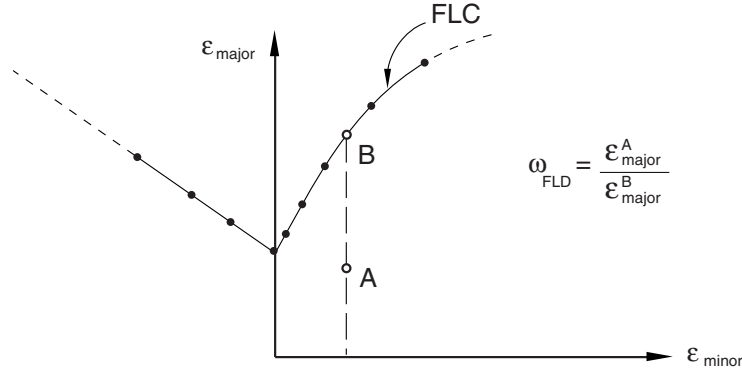
Figure 24.2.2–1 Forming limit diagram (FLD).
