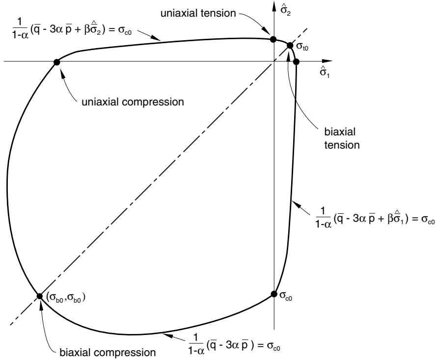
Figure 23.6.3-9 Yield surface in plane stress.
