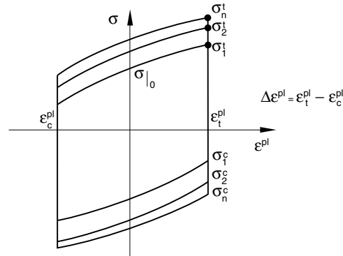
Figure 23.2.2-7 Symmetric strain cycle experiment.
