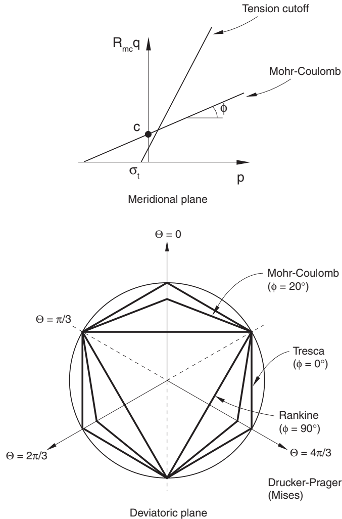
Figure 23.3.3-2 Mohr-Coulomb and tension cutoff surfaces in meridional and deviatoric planes.
