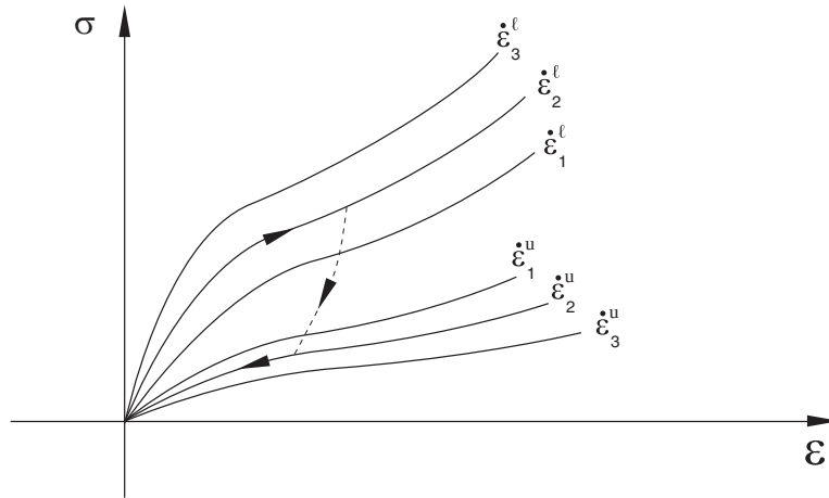
Figure 23.4.1–3 Rate-dependent loading/unloading.
