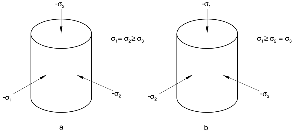
Figure 23.3.1-9 a) Triaxial compression and b) tension.
