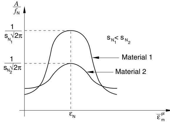
Figure 23.2.9–3 Nucleation function A/f_N .
