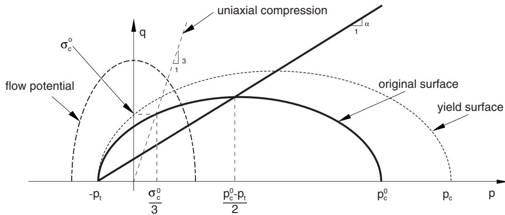
Figure 23.3.5-1 Crushable foam model with volumetric hardening: yield surface and flow potential in the p - q stress plane.
