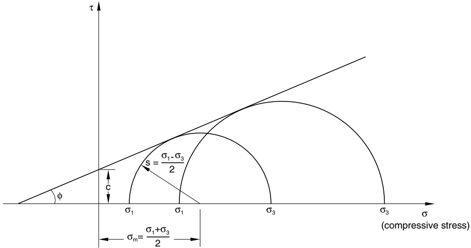
Figure 23.3.1–11 Mohr-Coulomb failure model.
