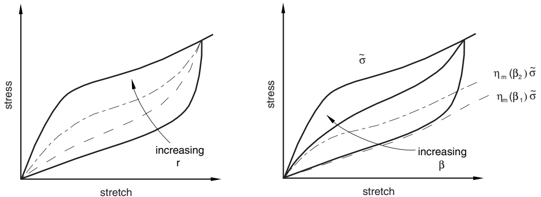
Figure 22.6.1-3 Qualitative dependence of damage on material properties.
