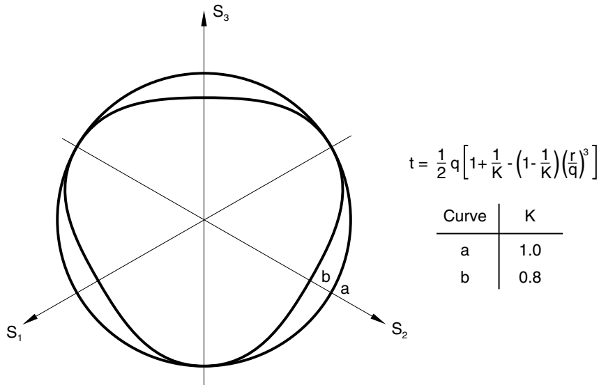
Figure 23.3.2–2 Typical yield/flow surfaces in the deviatoric plane.
