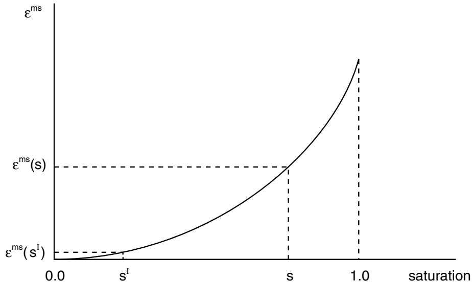
Figure 26.6.6-1 Typical volumetric moisture swelling versus saturation curve.
