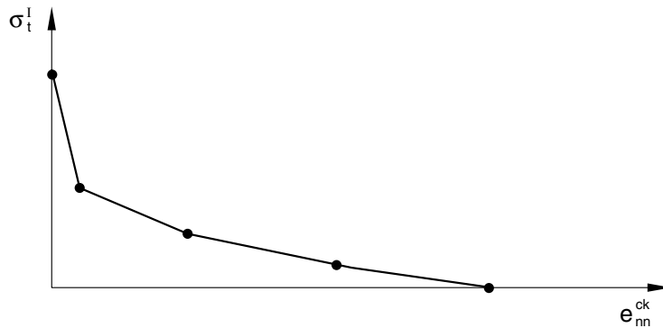
Figure 23.6.2–1 Postfailure stress-strain curve.
