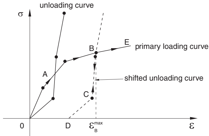
Figure 23.4.1-9 Shifted curve unloading.
