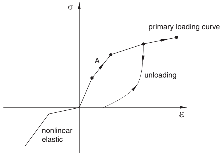
Figure 23.4.1–10 Different uniaxial models in tension and compression.
