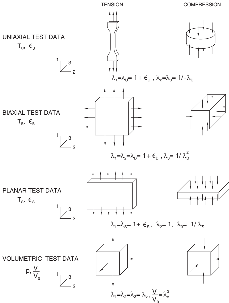
Figure 22.5.1–2 Schematic illustrations of deformation modes.
