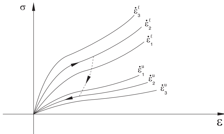
Figure 22.9.1–1 Rate-dependent loading/unloading stress-strain curves.
