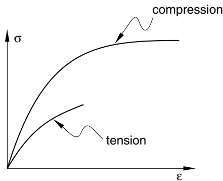
Figure 23.2.10–1 Typical stress-strain response of gray cast iron under uniaxial tension and uniaxial compression.
