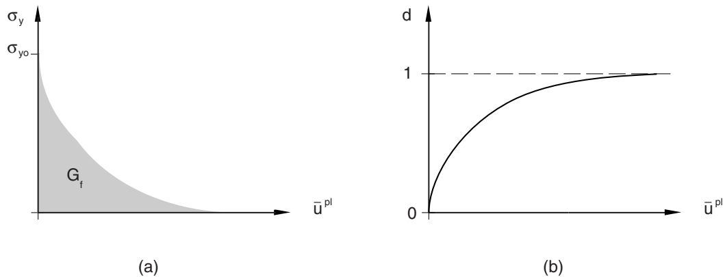
Figure 24.2.3–3 Energy-based damage evolution with exponential law: evolution of (a) yield stress and (b) damage variable.
