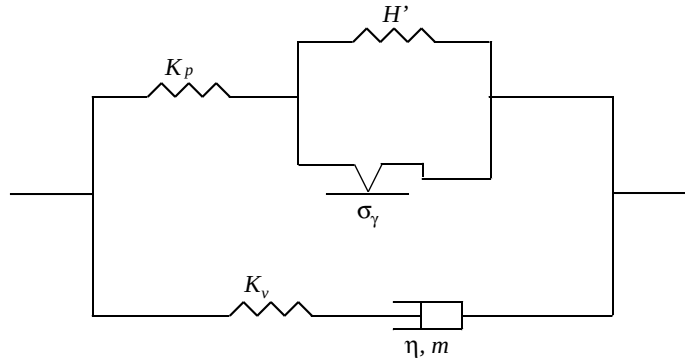
Figure 23.2.11-1 One-dimensional idealization of the two-layer viscoplasticity model.
