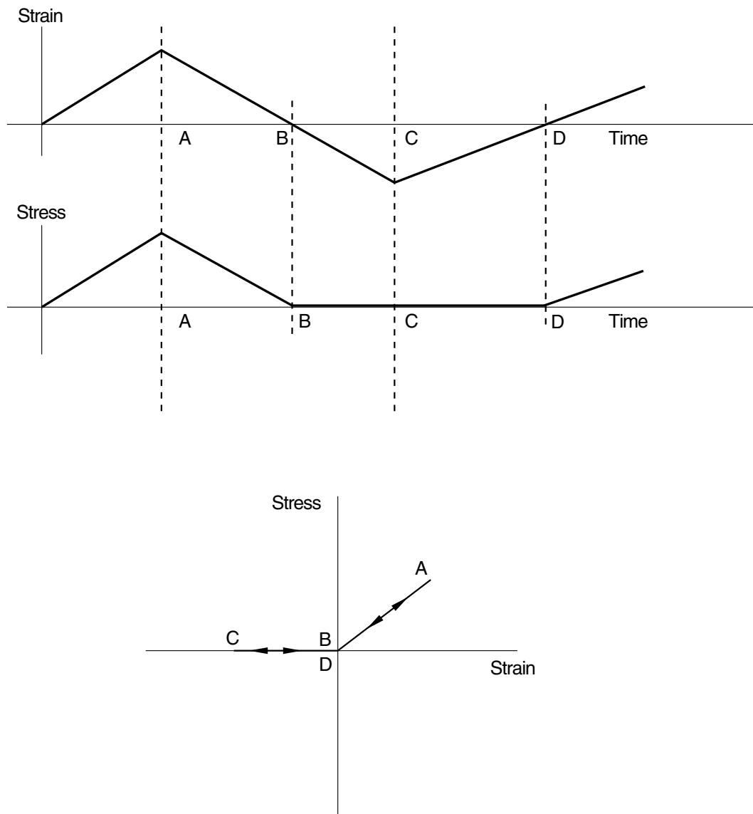
Figure 22.2.2-1 A no compression elastic case with an imposed strain cycle.
