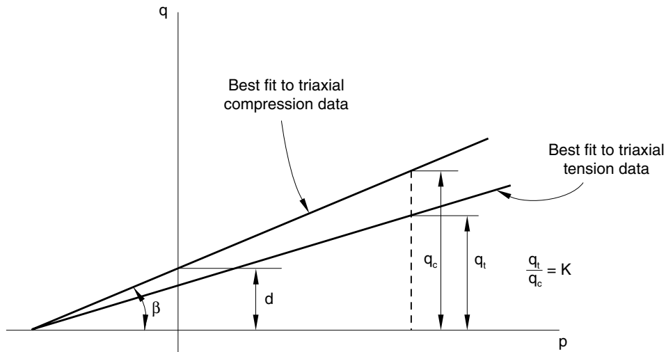
Figure 23.3.1–10 Linear model: fitting triaxial compression and tension data.
