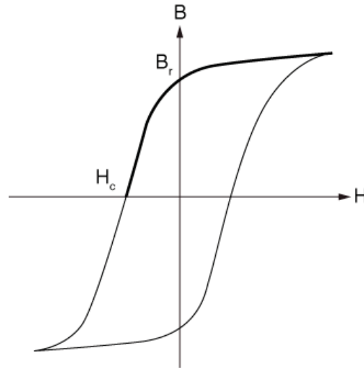
Figure 26.5.3-2 Remanence and coercivity in permanent magnets.
