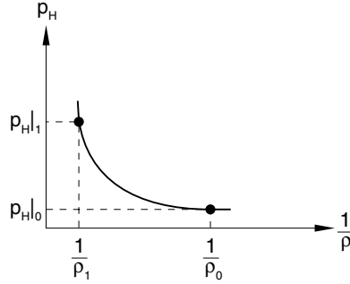
Figure 25.2.1-1 A schematic representation of a Hugoniot curve.
