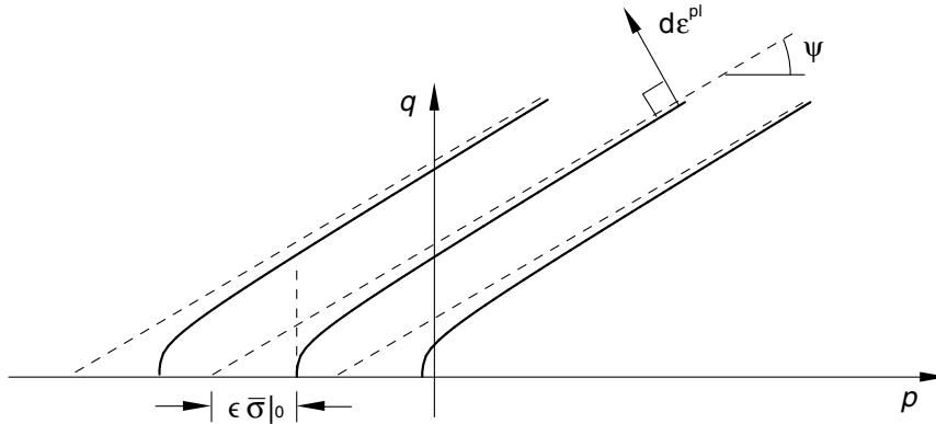
Figure 23.3.1–6 Family of hyperbolic flow potentials in the p - q plane.
