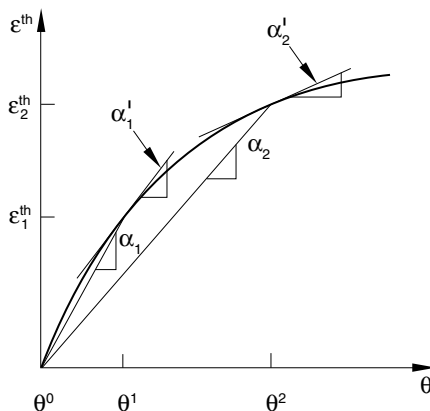
Figure 26.1.2–1 Definition of the thermal expansion coefficient.
