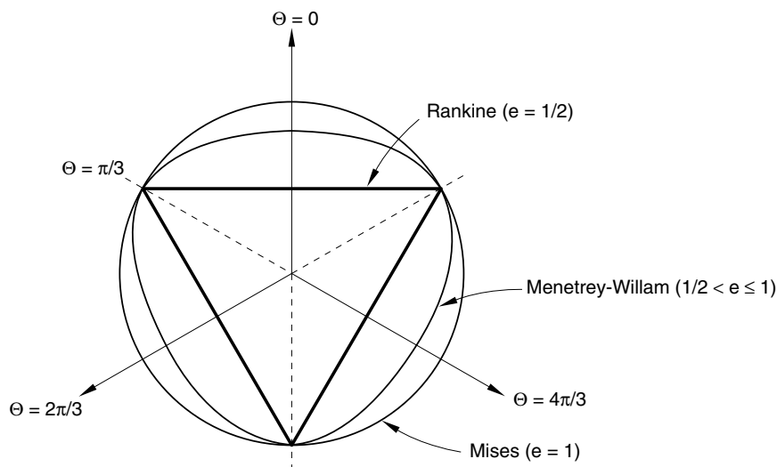
Figure 23.3.3–4 Menetrey-Willam flow potential in the deviatoric stress plane.
