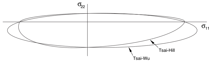
Figure 22.2.3-2 Tsai-Hill versus Tsai-Wu failure envelope ( I_F = 1.0 , F_{12} = 0.0 ).
