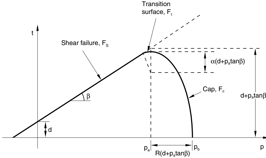
Figure 23.3.2–1 Modified Drucker-Prager/Cap model: yield surfaces in the p - t plane.
