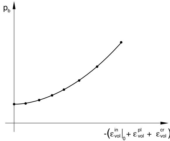
Figure 23.3.2–3 Typical Cap hardening.
