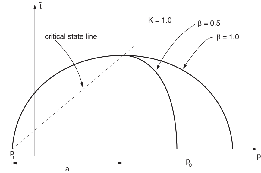
Figure 23.3.4-1 Clay yield surfaces in the p - \tilde{t} plane.
