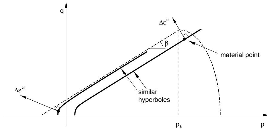
Figure 23.3.2-7 Cohesion creep potentials in the p - q plane.
