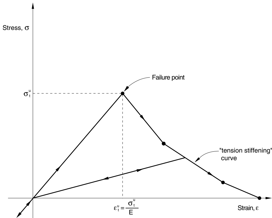
Figure 23.6.1–1 "Tension stiffening" model.
