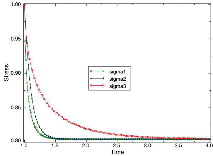
Figure 22.8.2-2 Normalized stress relaxation curves for three different strain levels.
