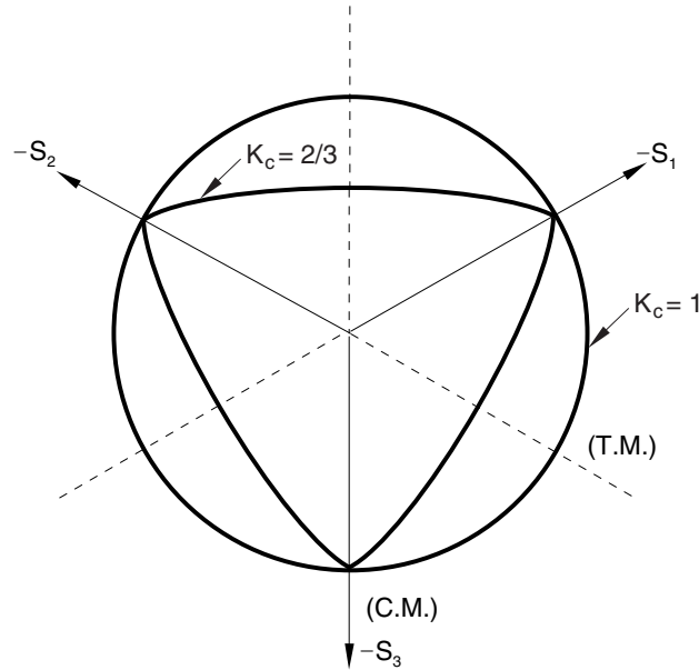
Figure 23.6.3–8 Yield surfaces in the deviatoric plane, corresponding to different values of K_c .
