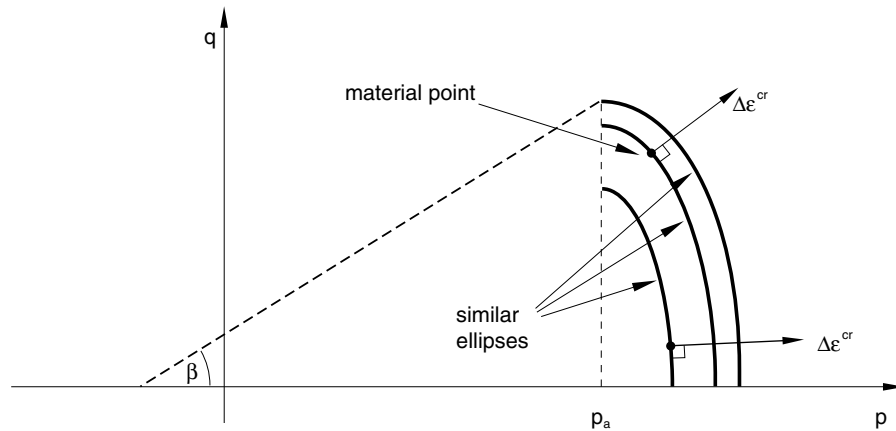
Figure 23.3.2-8 Consolidation creep potentials in the p - q plane.
