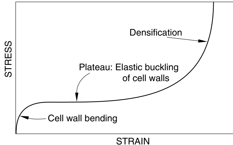
Figure 22.5.2–1 Typical compressive stress-strain curve.
