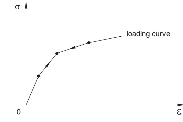
Figure 23.4.1–2 Nonlinear elastic rate-independent loading.
