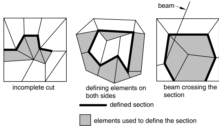
Figure 4.1.3-3 Invalid section definitions.
