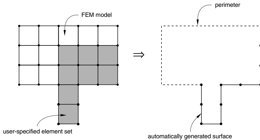
Figure 2.3.2–2 Automatic free surface generation.
