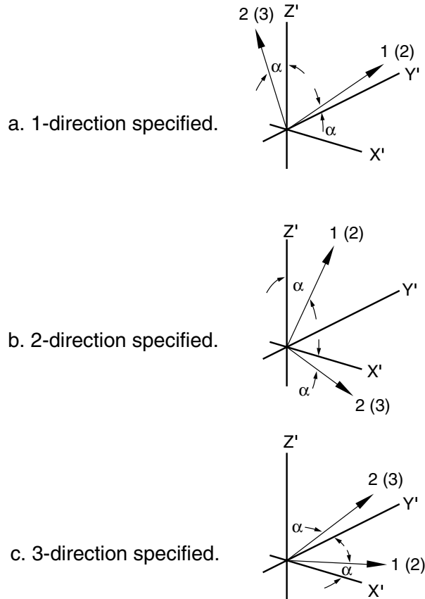
Figure 2.2.5–2 Specifying rotation about a local axis for contact surfaces in Abaqus/Standard, shells, membranes, composite solids, and (in parentheses) gasket elements.
