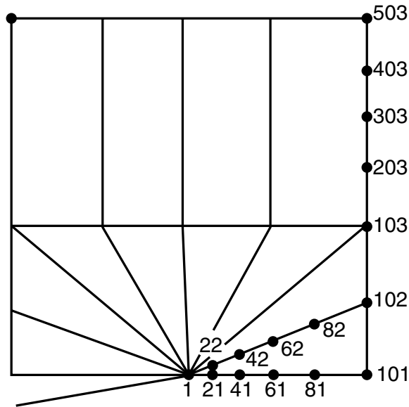
Figure 2.1.1-12 Node fill used in a singular problem.
