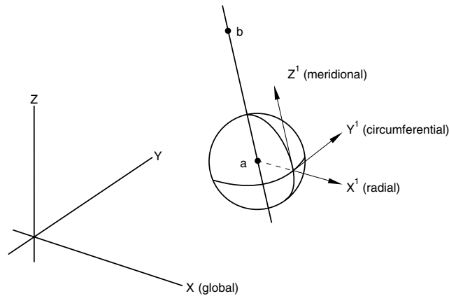
Figure 2.1.5–3 Spherical transformation.
