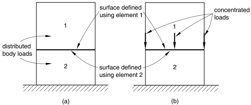
Figure 4.1.3-4 Total force in the section.
