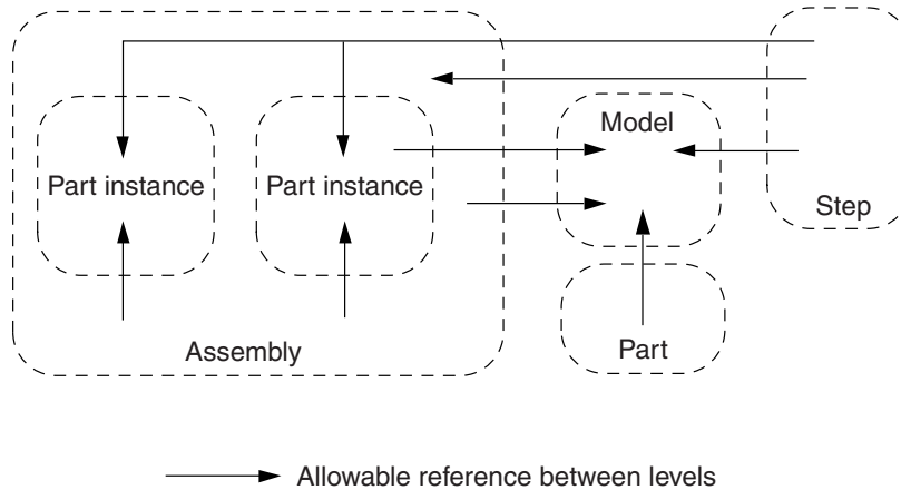
Figure 2.9.1–4 Allowable references between levels.
