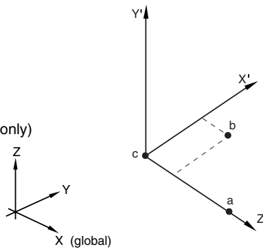
Figure 2.2.5–1 Orientation systems.
