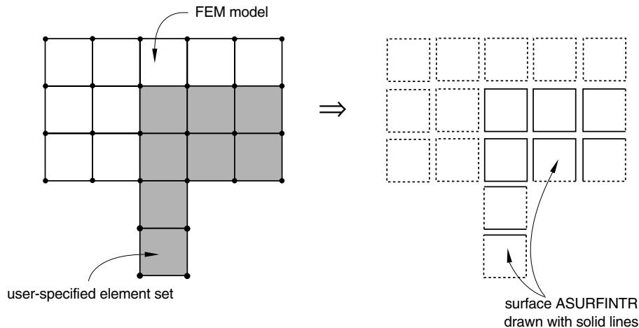
Figure 2.3.2–3 Automatic interior surface generation.
