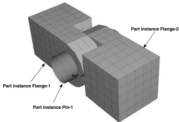
Figure 2.9.1–1 The hinge assembly.
