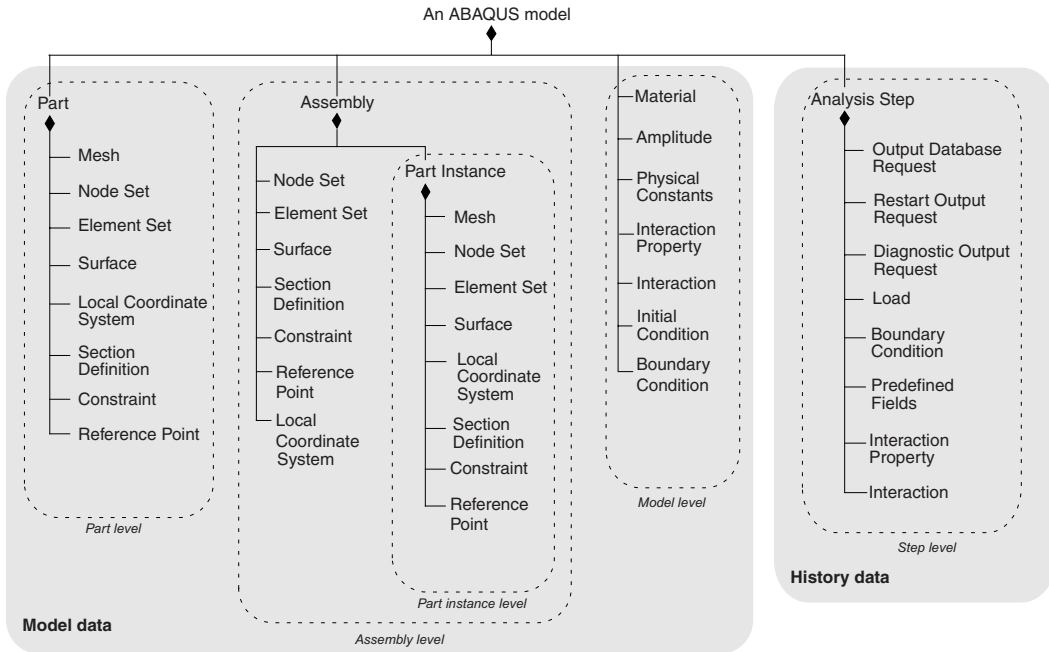
Figure 2.9.1–3 Organization of a model defined in terms of an assembly of part instances.
