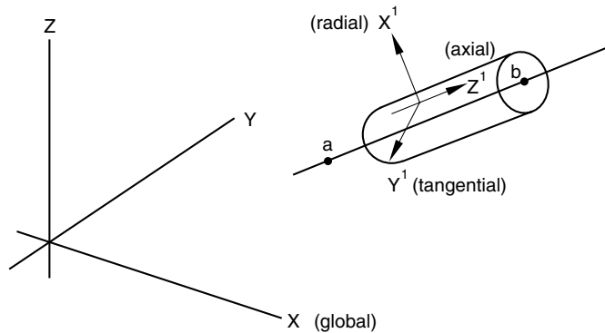
Figure 2.1.5–2 Cylindrical transformation.
