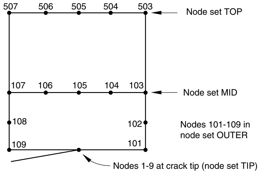
Figure 2.1.1–11 Node fill used in a singular problem.
