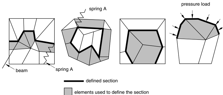
Figure 4.1.3–2 Valid section definitions.
