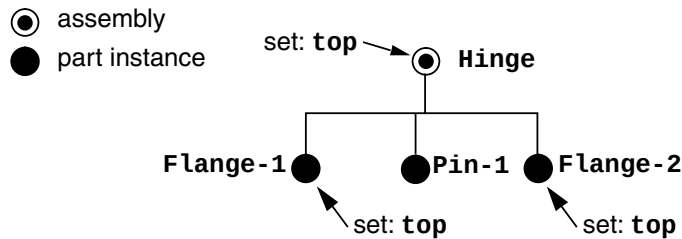
Figure 2.9.1–2 The organization of the Hinge assembly.
