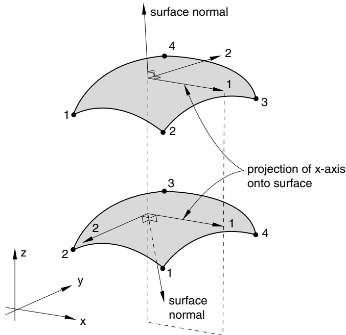
Figure 1.2.2–1 Default local surface directions.
