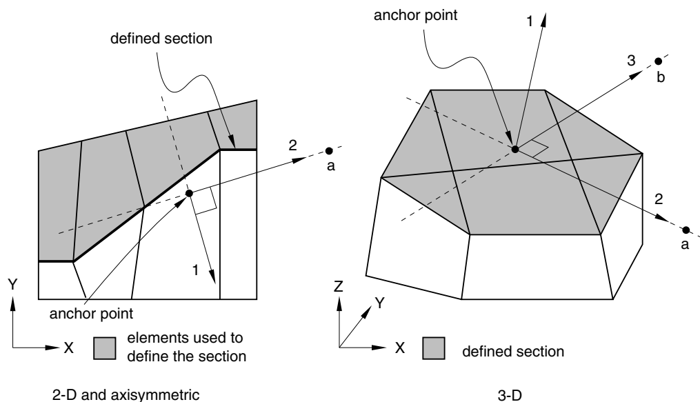
Figure 2.5.1–1 User-defined local coordinate system.
