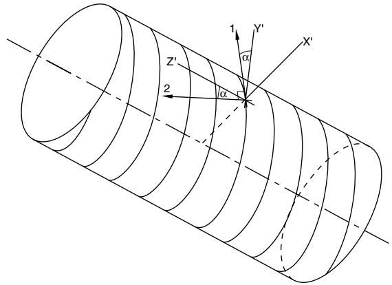
Figure 2.2.5–4 Spiral-wound cylindrical shell layer: material orientation example.
